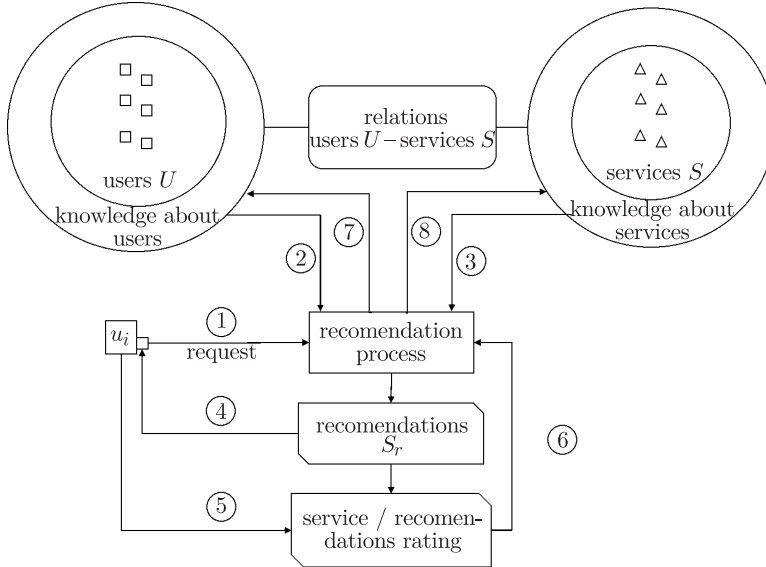
Figure 1. General scheme of the recommendation system
