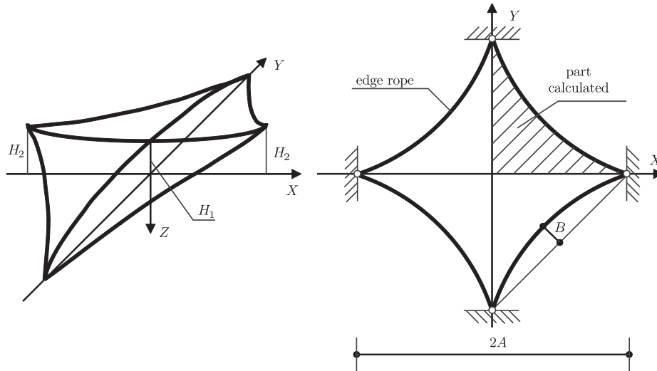
Figure 4. Roof geometry
