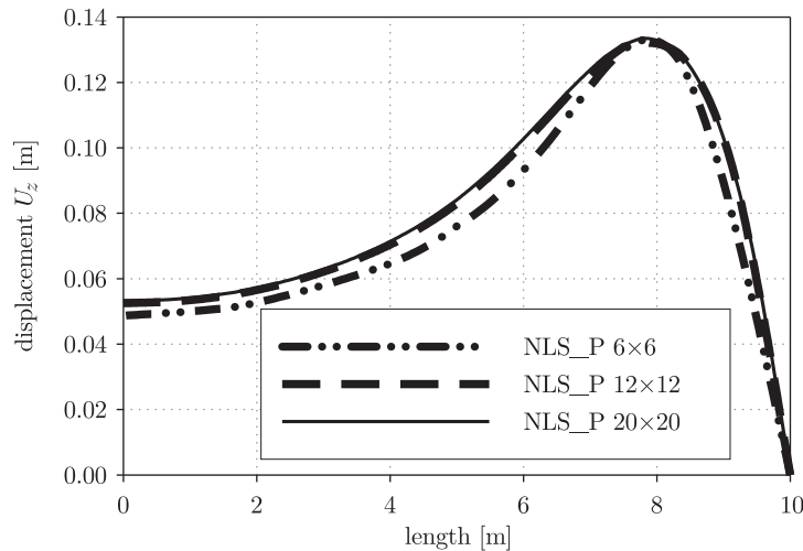
Figure 5. Convergence analysis of FE mesh – vertical displacement along X axis
